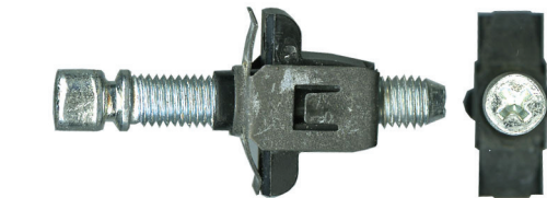
FA 1790 $2.50 Headlight Adjusting Nut and 1/4-28x1-1/2 Screw - Discontinued
