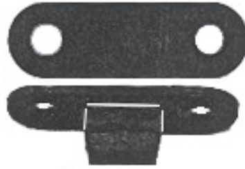
FA 2411 $0.80 Headlight Rim to Grille Retainer
