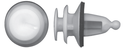
FA 4318 $1.00 Trim Panel Retainer GM
