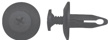
FA 2118 $0.90 Hole Dia. .250 Panel Range .100-.240 Flange OD .700
