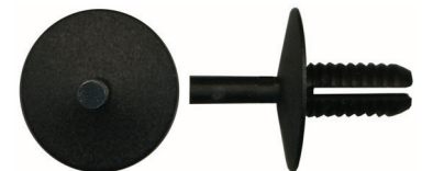
FA 4720 $0.75 1989 on BMW Head 20mm stem lgth 15mm fits 6.3 mm hole
