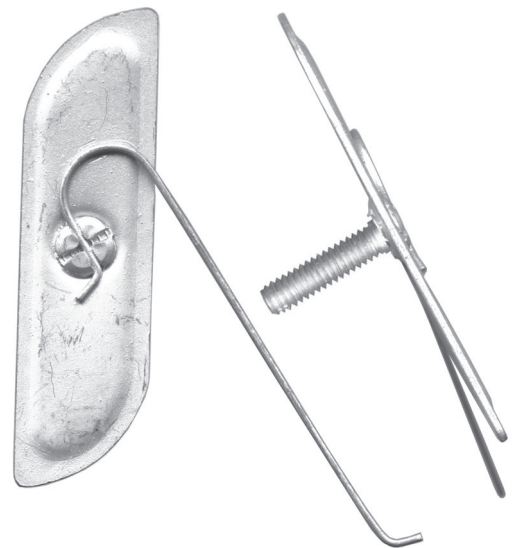
FA 4534 $2.80 T-Bolt 1024x3/4 stud 2-17/32" length 11/16" width
