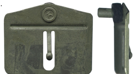
FA 4557 $3.90 Moulding Clip 85-91 Skylark
