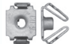
FA 4404 $2.95 M6-1.0 Push Nut 96/ GM G,S, & T Trucks
