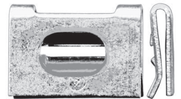
FA 2566 $0.45 #8 U-Nut Range .30-.40 Self Aligning
