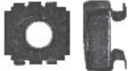
FA 923 B $0.95 5/16-18 Caged Nut, Blk.028-.056 P.R.
