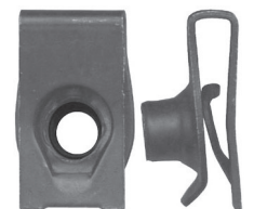
FA 691 $0.85 1/4-20 U-Nut .025-.150 Panel
